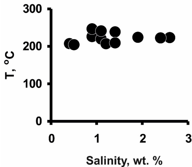
Figure 9. Temperature versus salinity diagram for ore-forming fluids (sample N1).
