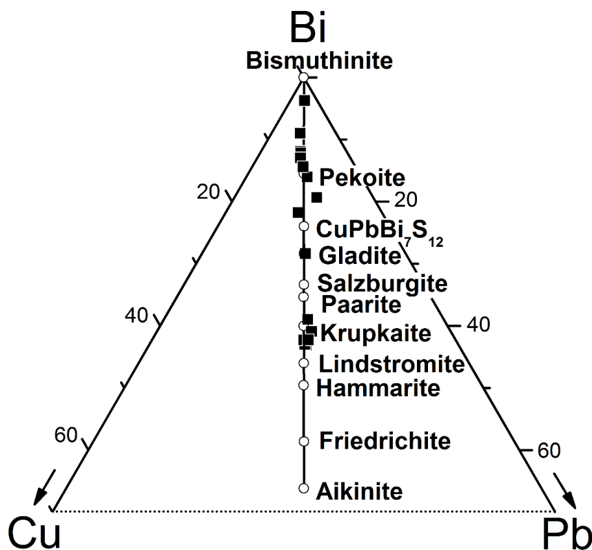
Figure 5. Compositional data for bismuthinite derivatives plotted on a Cu-Pb-Bi ternary diagram (atom %).
