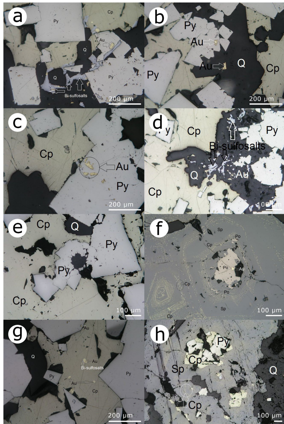
Figure 2. Photomicrographs in reflected light showing textural aspects of the assemblage containing native gold and Bi-sulfosalts. (a) Native gold–Bi-sulfosalts–sulfides assemblage. (b) Native gold inclusion in pyrite and in euhedral quartz. (c) Native gold inclusion in pyrite. (d) Pyrite associated with chalcopyrite and Bi-sulfosalts within quartz. (e) Radiating aggregates and euhedral crystals of pyrite inclusion in chalcopyrite. (f) Pyrrhotite as a small crystal associated with the native gold on growth surfaces within sphalerite, sphalerite contains exsolutions of chalcopyrite and of pyrrhotite. (g) Chalcopyrite with inclusions of native gold and Bi-sulfosalts, quartz pyrite. (h) Sphalerite as coarse aggregates with abundant chalcopyrite exsolutions, containing euhedral crystals of pyrite and chalcopyrite. Abbreviations: Au—native gold; Cp—chalcopyrite; Py—pyrite; Po—Pyrrhotite; Q—quartz.
